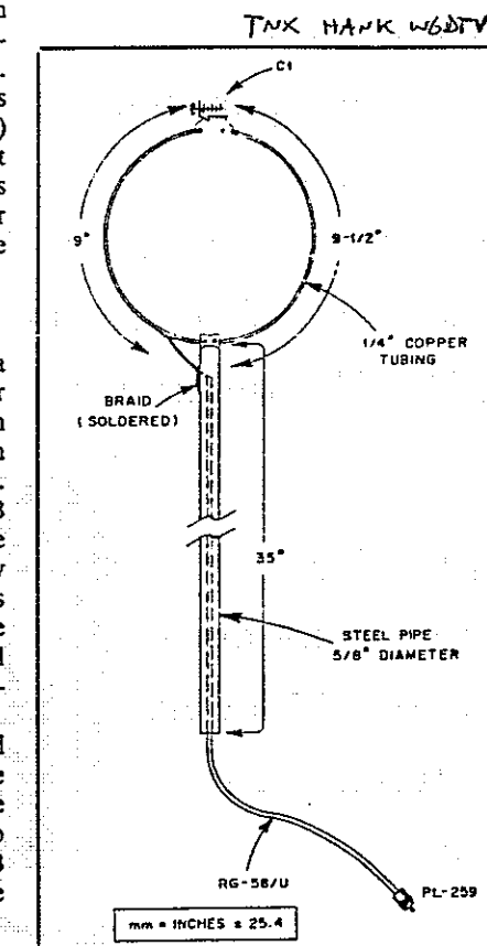
Fig. 1 — Construction of the Fox Fixer.
